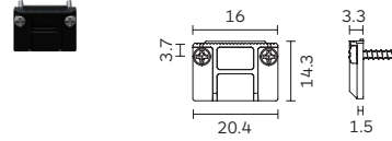
T258 Metal Sheet End Cap for 2STC Track
