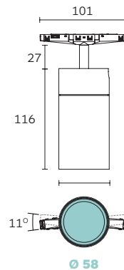
Flexible adaptor for curved track
