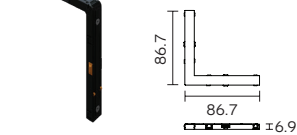
T262 Vertical Corner Joint Cover
