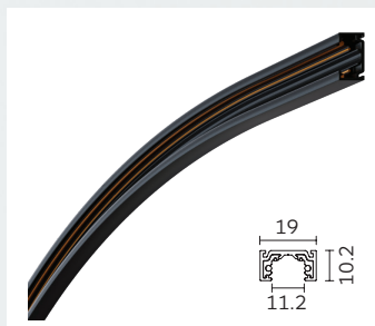
Horizontal curved track
