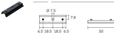
T255 Bracket
