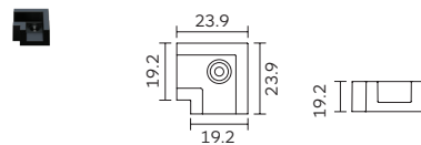
T255 Bracket
